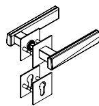
JETTE VISION RG Schlüssellosetten PZ JETTE VISION RG Roses PZ
